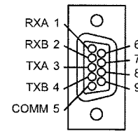
RS-485 (4-wire) DB9-F
